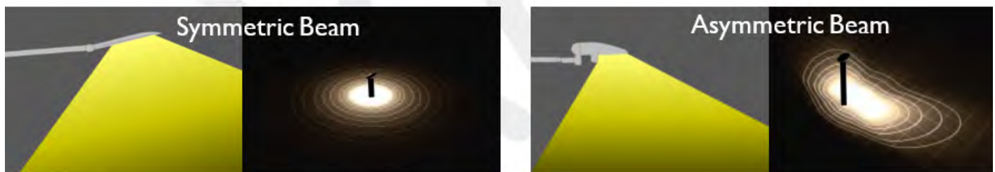
Figure 27 - Asymmetric and symmetric beam patterns © Darkscape Consulting
