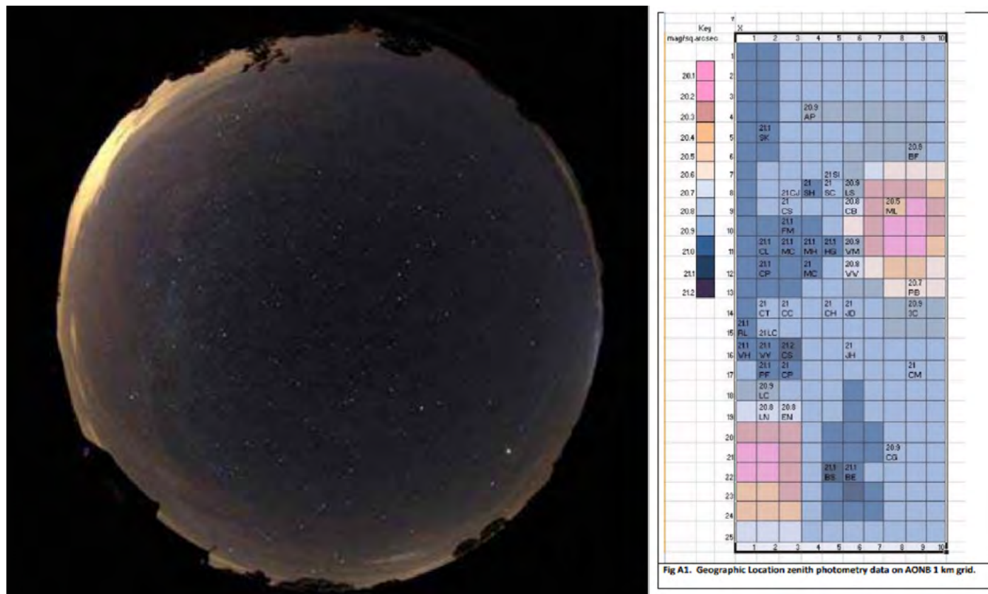
Figure 5 - Image of the Milky Way above the Malvern Hills National Landscape. Location of data points shown in grid with SQM values. © Chris Baddiley and from Malvern Hills State of the AONB report.
