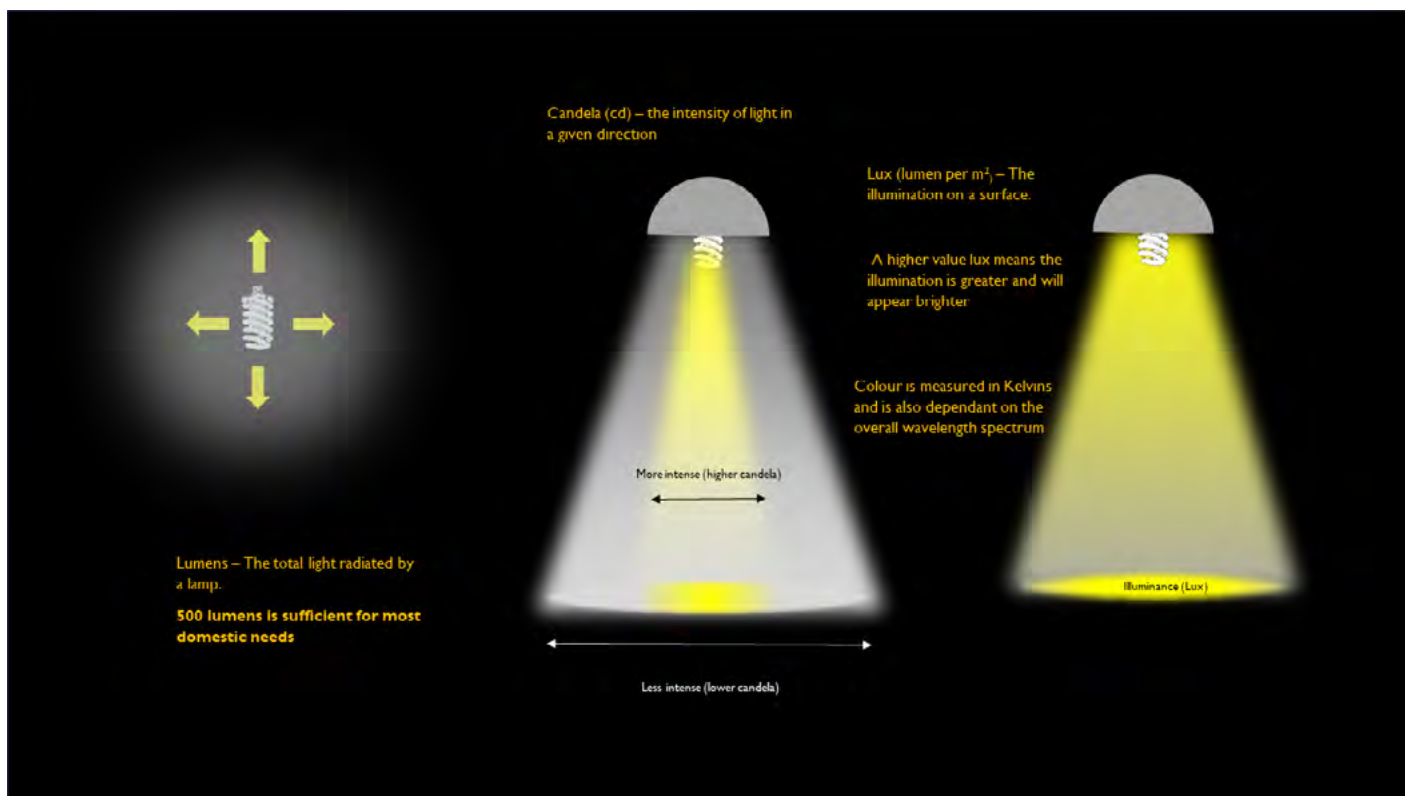
Figure 10 - The properties of light © Darkscape/South Downs National Park Authority Technical Advice Note
