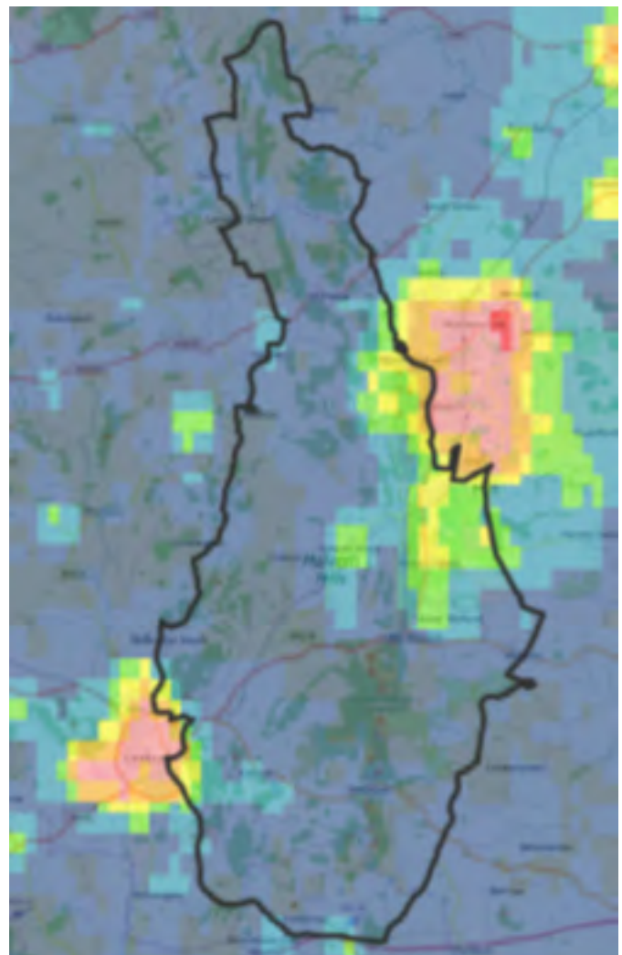
Figure 6 - Dark Sky Discovery Sites over CPRE data. Mathon (Top), Castlemorton (Bottom)
