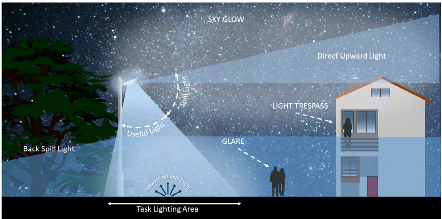
Figure 8 – Sources of light pollution.
