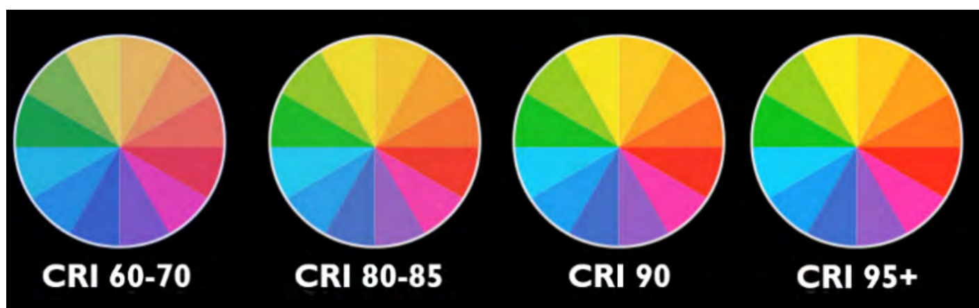
Figure 14 - Colour Rendition Index (CRI).
