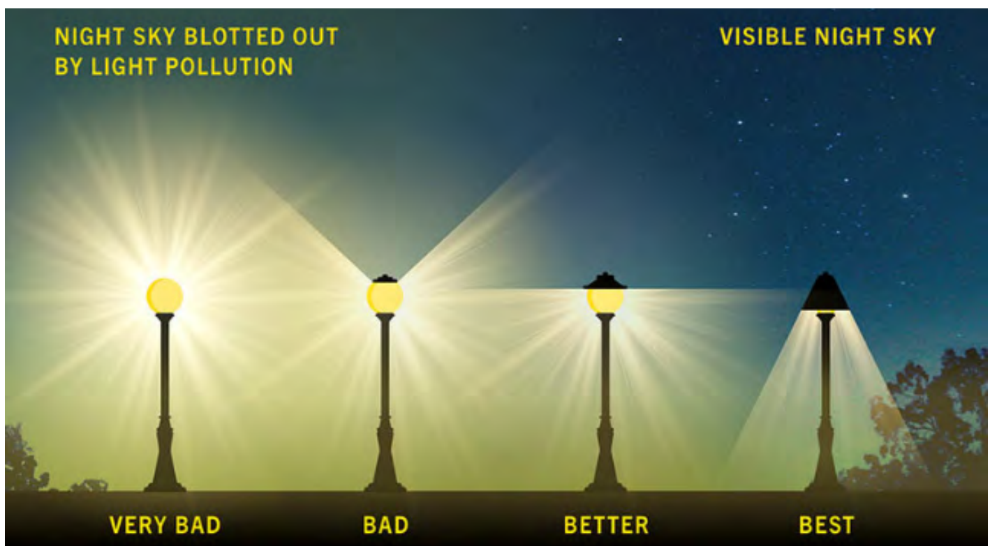
Figure 18 - The impacts of upward light - The International Dark Sky Association
