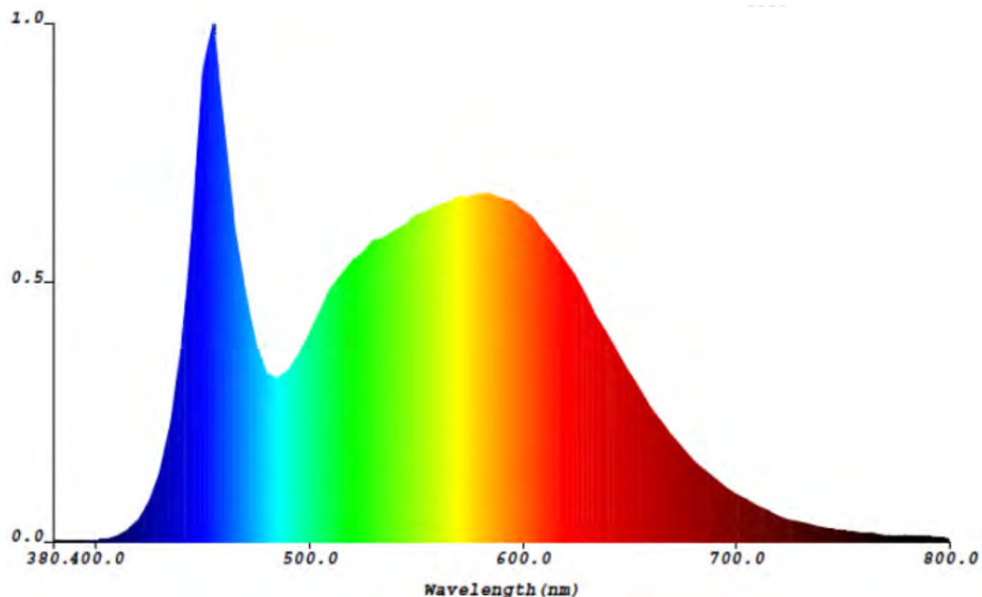
Figure 13 - The colour spectrum from a 5000K lamp with a prominent blue peak which exacerbates light pollution.
