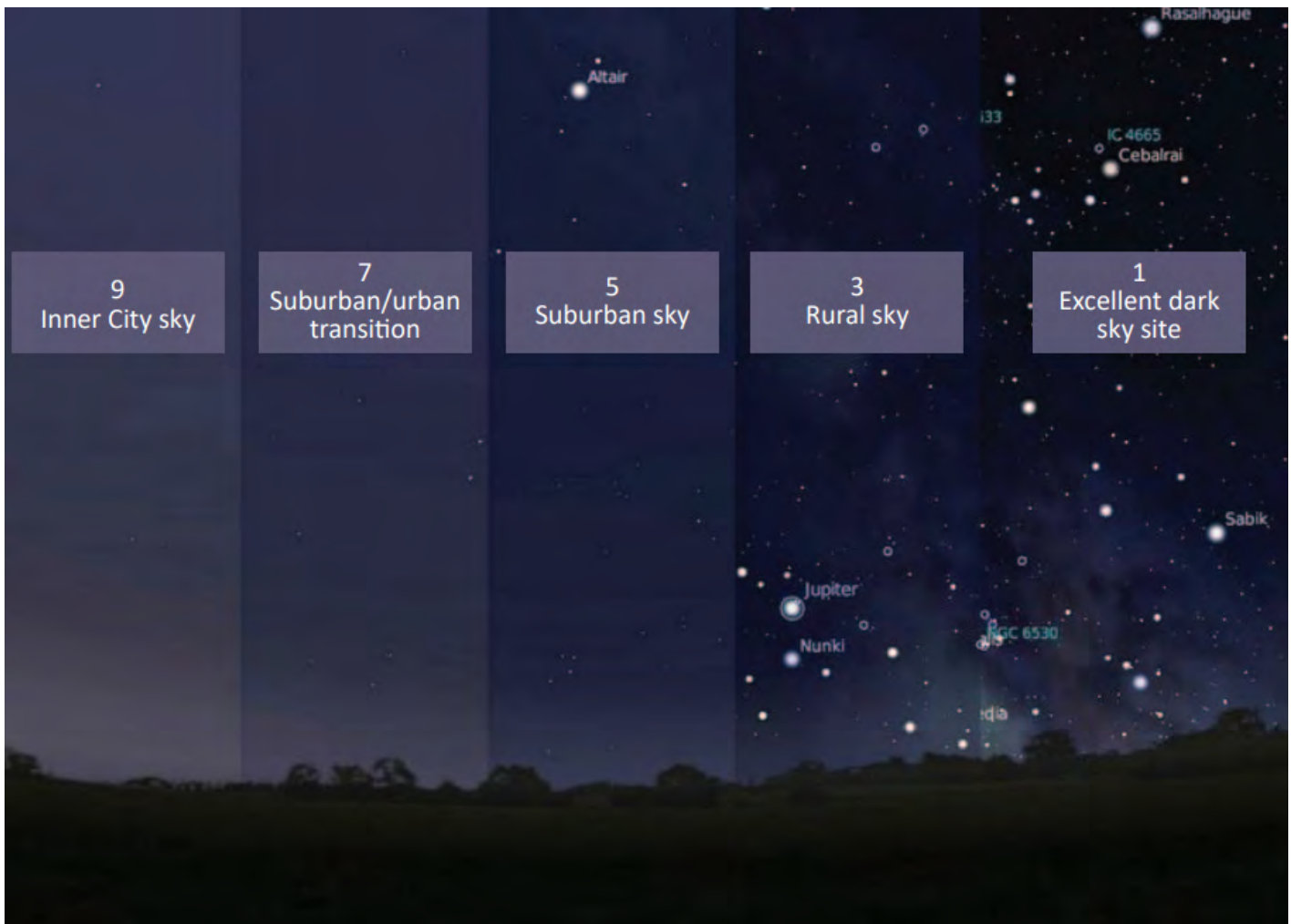
Figure 3 - Bortle Scale using Stellarium Software. The scale is named after John E. Bortle, who published it for the first time in the February 2001 issue of the Sky and Telescope magazine.
