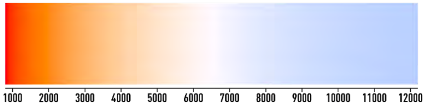
Figure 11 - The Kelvin Scale (K)
