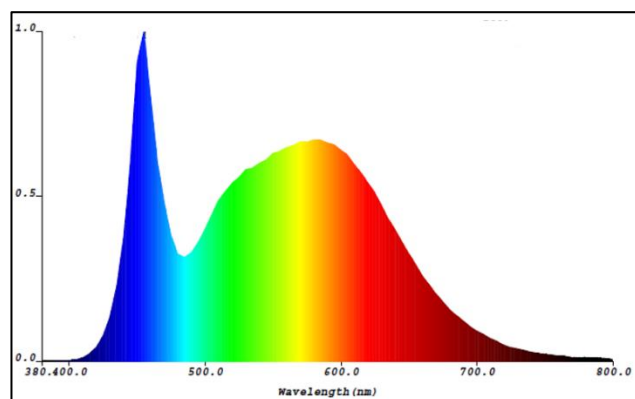
Figure 13 - The colour spectrum from a 5000K lamp with a prominent blue peak which exacerbates light pollution.
