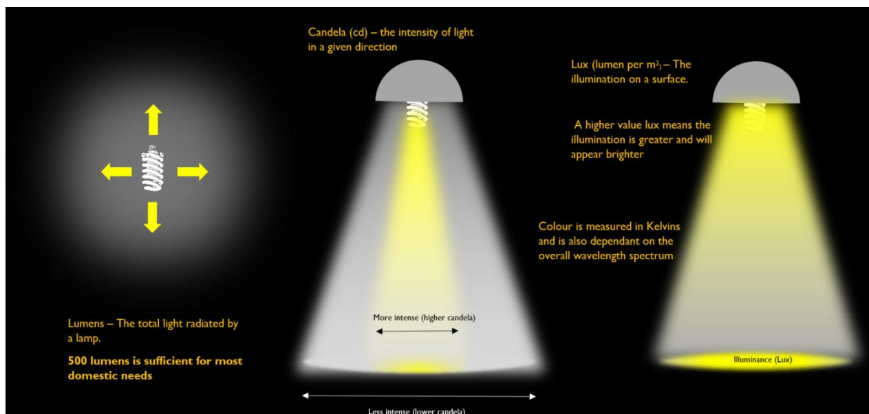
Figure 10 The properties of light. Credit Darkscape/South Downs National Park Authority Technical Advice Note
